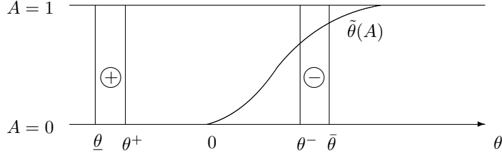
Figure 6: \theta^+ , \theta^- , \underline{\theta} and \bar{\theta}
