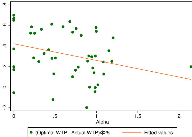
Figure 5: Subject-level Overconfidence as a Function of \alpha
