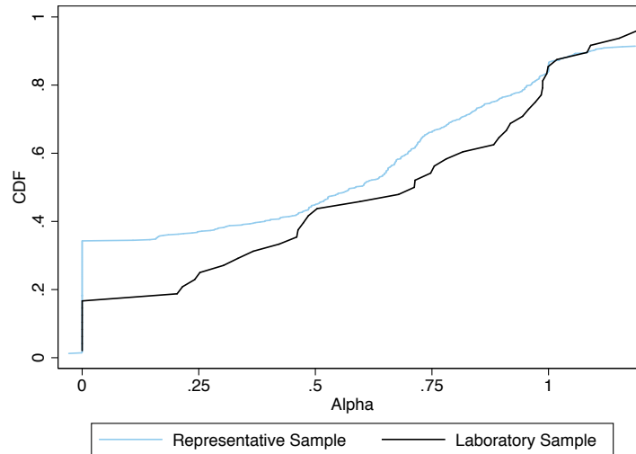
Figure 3: CDF of Alpha
