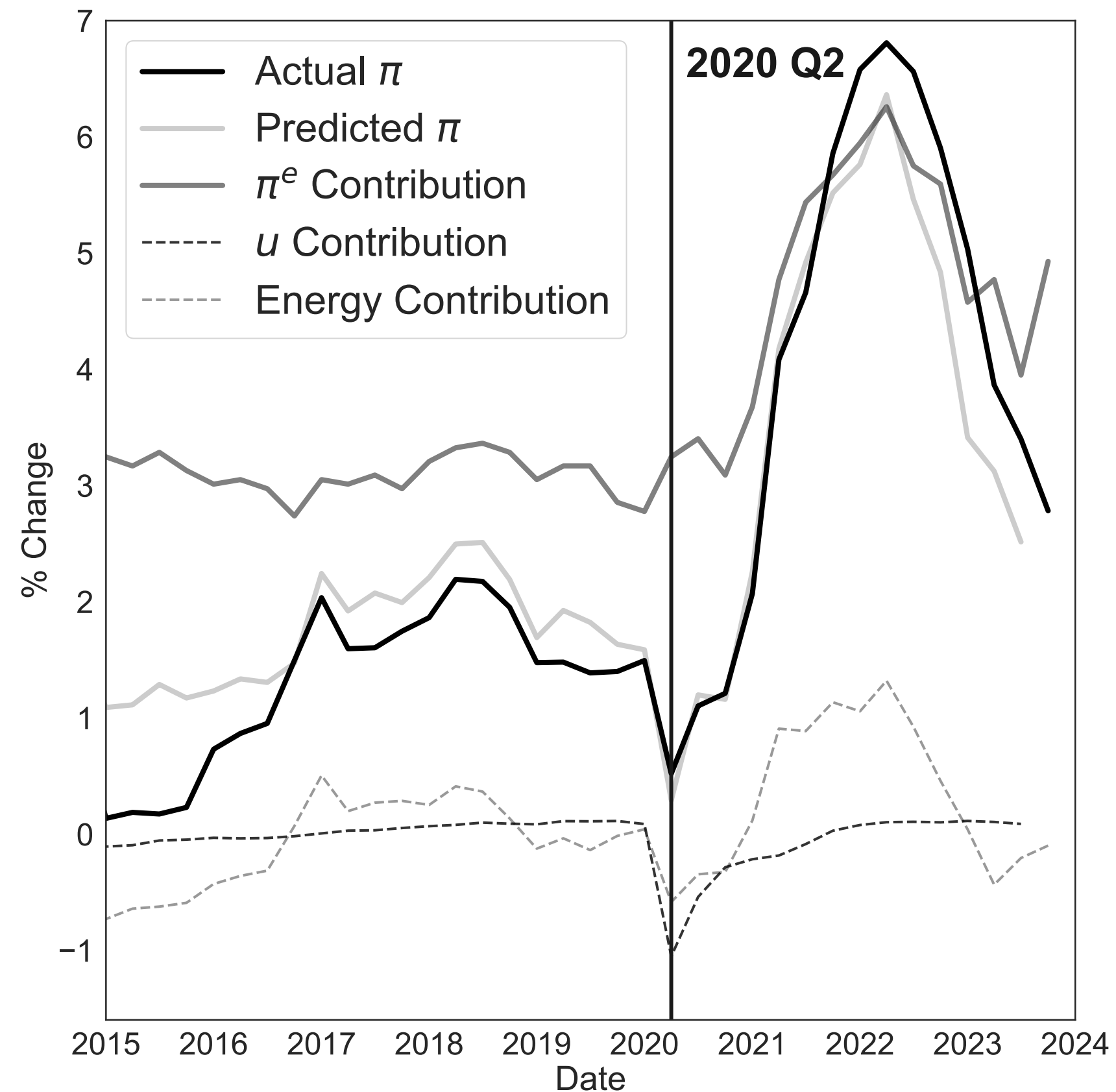
Figure 3: Predicting Post-2020 Inflation using Pre-2020 Phillips Curve
