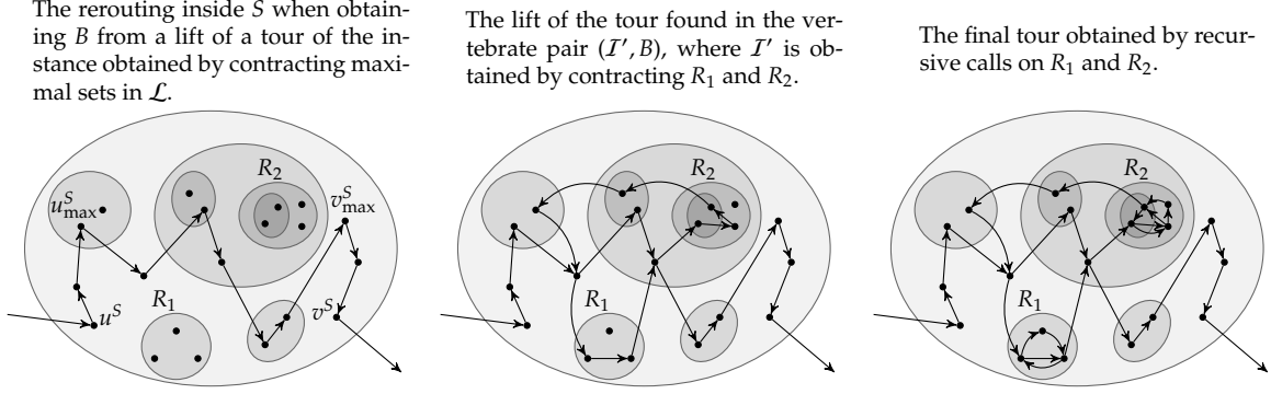
Figure 4: An illustration of the steps in the proof of Theorem 4.2. Only one maximal set S \in \mathcal{L} is shown.
