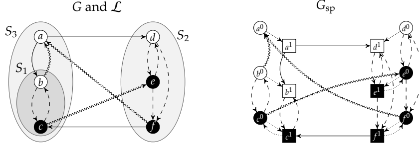
Figure 5: An example of the construction of G_{\text{sp}} . The vertices of the backbone are depicted in black. The nonsingleton sets in \mathcal{L} are S_1 , S_2 , and S_3 . Straight, swirly, and dashed edges correspond to various edge types in the construction.
