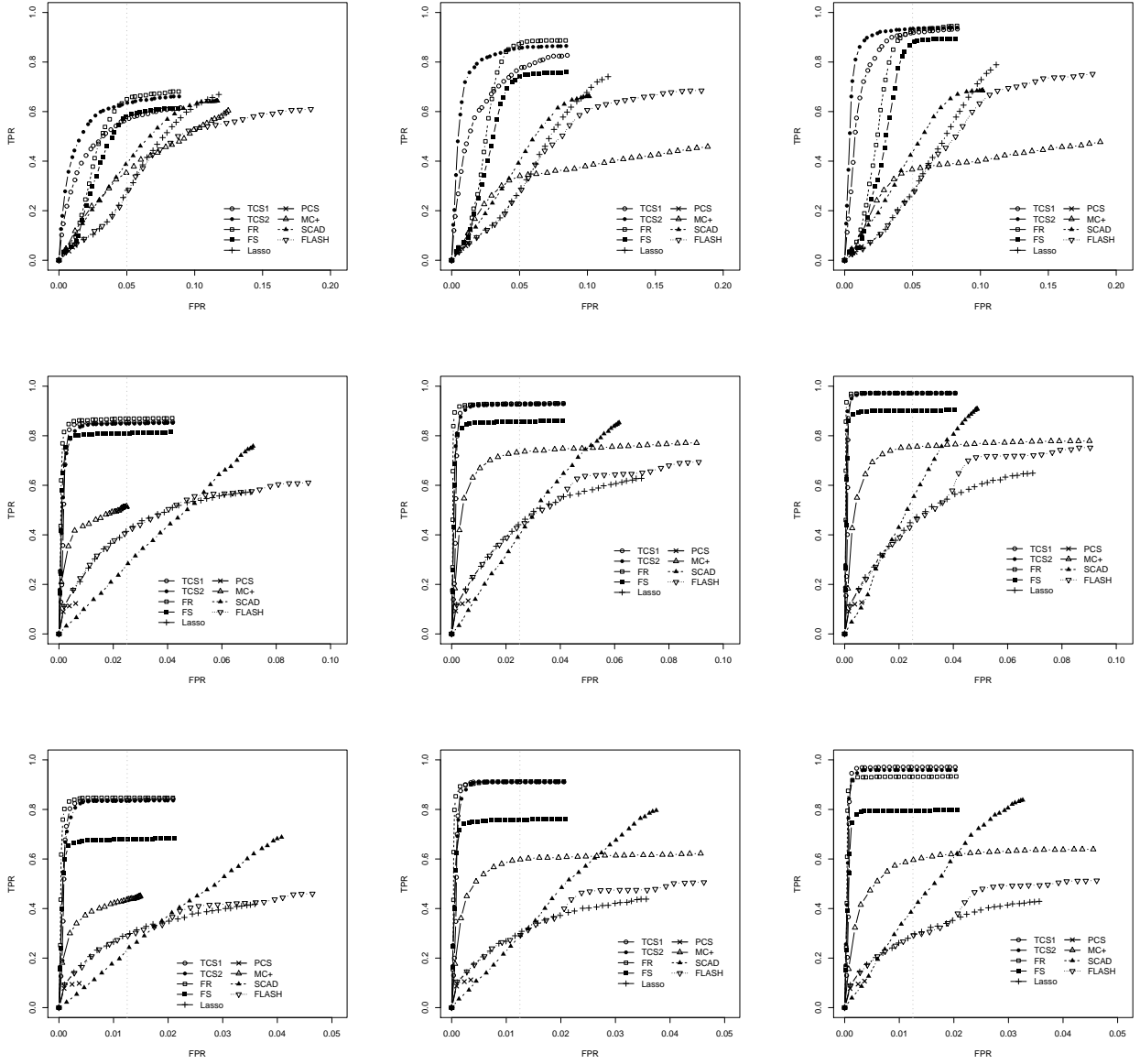
Figure 1: ROC curves for the simulation model (A) with n = 100 : TCS1 (empty circle), TCS2 (filled circle), FR (empty square), FS (filled square), Lasso (crossed circle) PC-simple algorithm (cross “x”), MC+ (empty triangle), SCAD (filled triangle) and FLASH (reversed triangle); FPR = 2.5|S|/p (vertical dotted); first row: p = 500 , second row: p = 1000 , third row: p = 2000 ; first column: R^2 = 0.3 , second column: R^2 = 0.6 , third column: R^2 = 0.9 .
