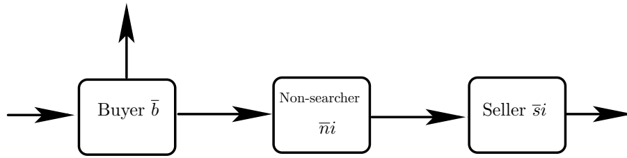
Figure 1: Life-cycle. No Short-Sales, Search Spot Market.
